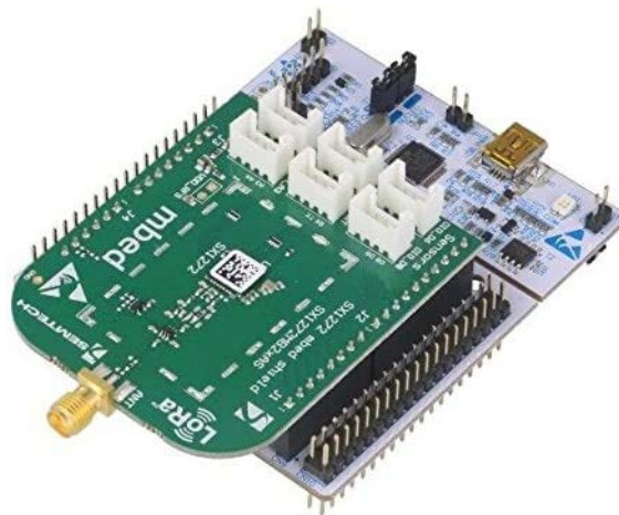
Figure 131: Boîtier P-NUCLEO-LRWAN1
