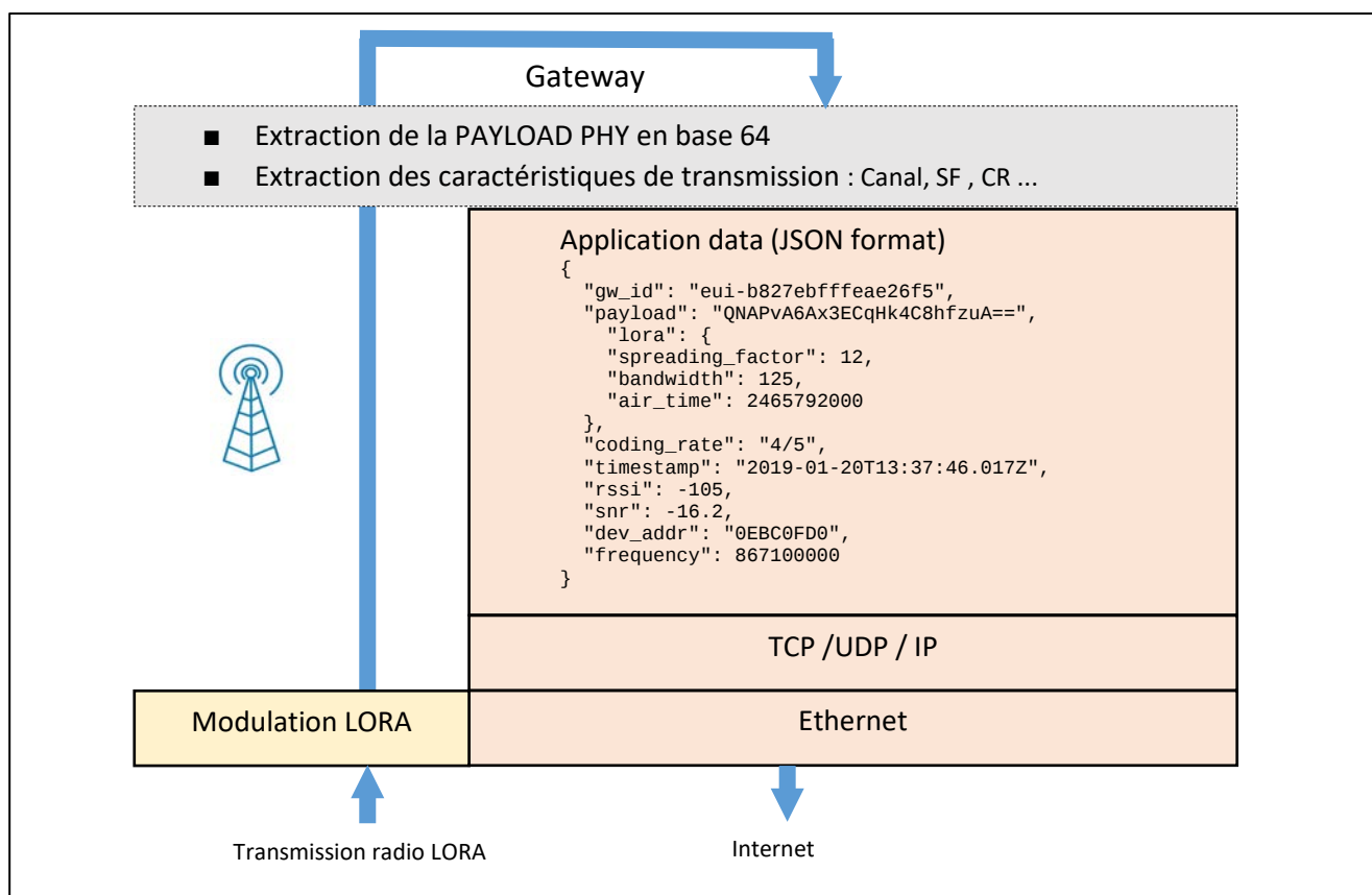
Figure 101: Gateway LORAWAN
