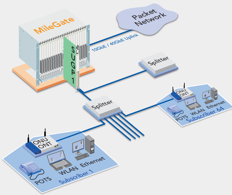
FTTH connections with MileGate SUGP1
