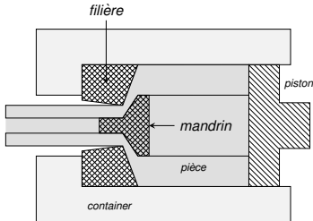
Mandrin flottant
