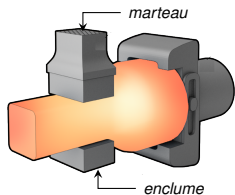
Forgeage libre
