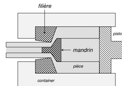
Mandrin flottant
