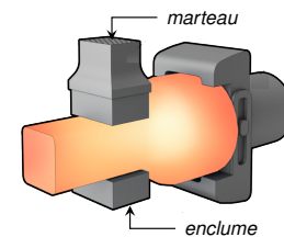
Forgeage libre
