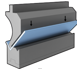
pliage
