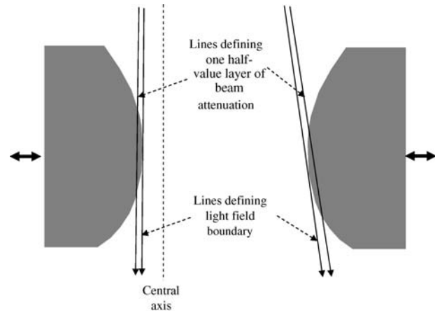
Figure A.2.1. The effect of curved leaf ends. For reasons of mechanical simplicity, most conventional MLCs use simple linear motion (as indicated by the bold double arrows). Here, one leaf is shown close to the central axis and the other farther from the central axis. If the leaves were not curved, there would be a sharp transition in crossing the central axis where the light field would be defined first at the top and then at the bottom of the collimator. The use of curved leaf ends causes the edge of the light field to differ from to the edge of the radiation field, which is typically defined by one half-value layer of attenuation. The discrepancy between the boundary defined by the light field and the radiation field is not constant with leaf position, but varies with position across the field. There is also significant leakage through the leaves when the leaves are in the “closed” position. In the “closed” position, opposed leaves might not touch because there is usually a small gap between the leaves. Curved leaf ends also degrade the penumbra of the field and make beam modeling in this region more difficult.
