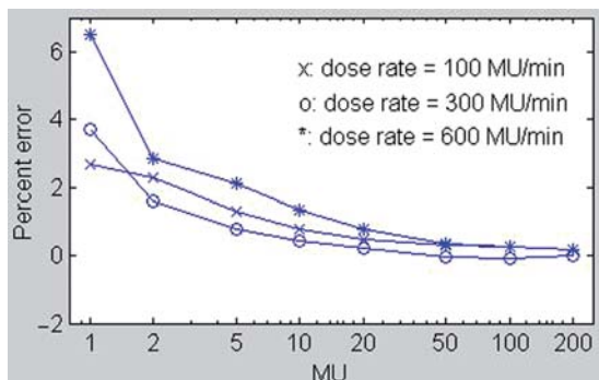
Figure A.2.5. Measurement of the error that can result when a small number of monitor units (MUs) are delivered multiple times. The abscissa represents MU per delivery. After each delivery, the beam is turned off. In all tests, a total of 1000 MU was delivered. Unlike conventional radiotherapy, small numbers of MUs are often delivered for different segments in IMRT. The error is generally larger for small numbers of MUs delivered at high absorbed-dose rates. (From Palta et al. , 2003; reproduced with permission.)
