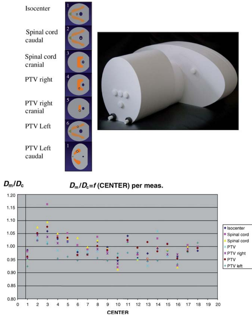
Figure A.2.10. Upper panel is the phantom developed by the GORTEC to compare the ratio of the measured absorbed dose to the computed absorbed dose at several positions for head-and-neck radiotherapy. The orange regions of interest indicate the target volume on each of the slices. About 20 % of the 126 TLD measurements from 18 centers did not agree within 5 % of the treatment-planning calculations. The spread of measurements within a center was much less than the spread of measurements between centers. (Figure courtesy of Milan Tomsej, St. Luc University Hospital, Brussels, Belgium.)
